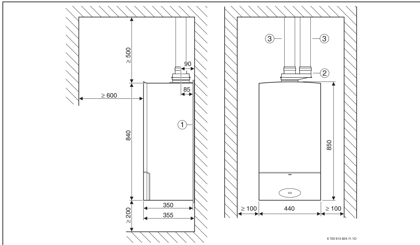
sl. 12 Ø 80/80 mm, ravan krov
