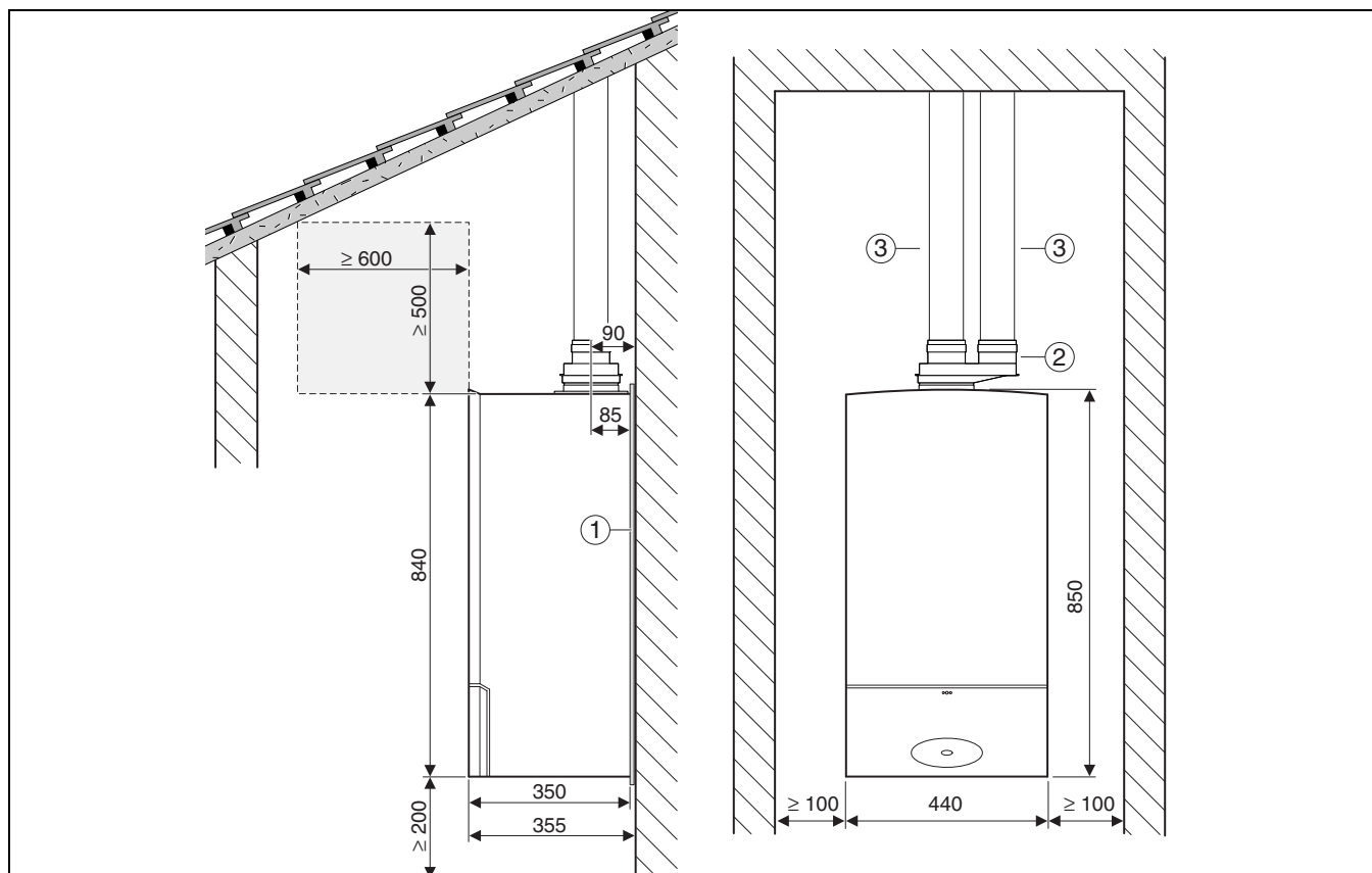
sl. 13 Ø 80/80 mm, kosi krov
